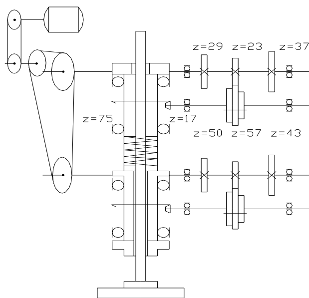
Figure 1. Kinematics diagram of lapping
