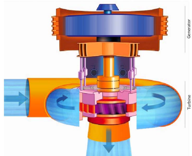
Figure 1. Cross-section view of a generating unit, update 10.04.13[1].
