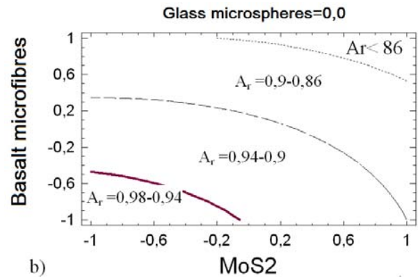
Figure 2. The estimation of PCM relative adherence the function of constituents concentration for various levels of response factors: a) MoS 2 =0; b) eglass microspheres=0.
