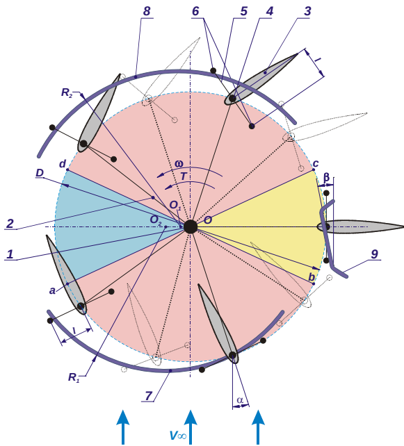
Figure 12. Differentiated orientation mechanism of blades.
