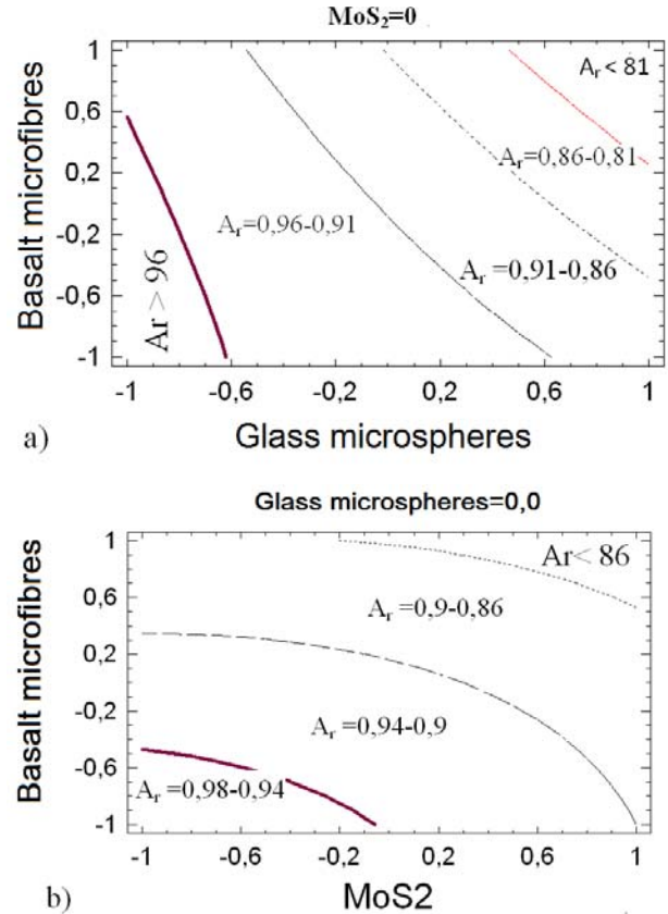
Figure 2. The estimation of PCM relative adherence the function of constituents concentration for various levels of response factors: a) MoS 2 =0; b) eglass microspheres=0.
