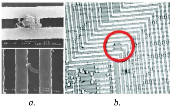
Figure 2. Defect images: (a) Bridging defects with low-resistance electrical behaviour on the top and high-resistance electrical behaviour on the bottom microphotograph, and (b) Open defect inside the circle [17]
