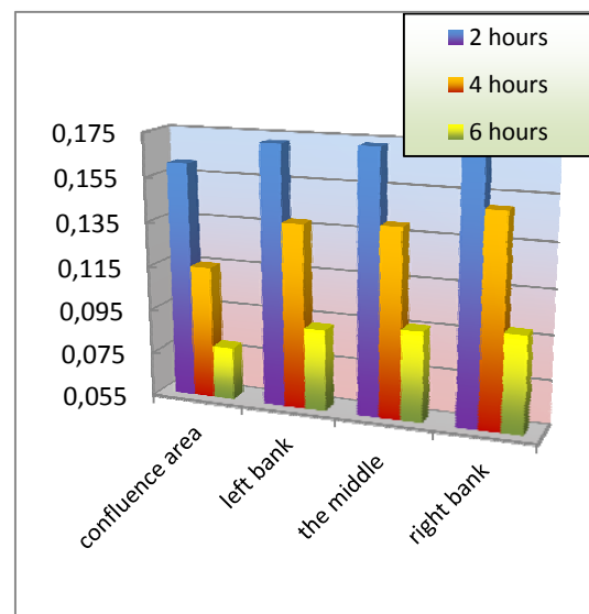
Figure 4. Temporal evolution of the iron concentrations field.
