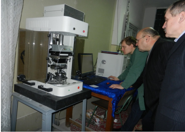
Figure 3. Aspects from the measurement of the coefficient of friction with the universal tribotester UMT2 (CETR ®, USA) with pin-on-disk configuration: 1 - dual sensor for friction and load, 2 - suspension, 3 - pin support, 4 - pin, 5 - disc, 6 - table- support for disc.
