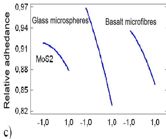
Figure 1. The estimation of PCM relative adherence the function of constituents concentration for level 0 (the concentration of basalt microfibres 4%): a) the response surface, b) the response levels and c) dominants effects.
