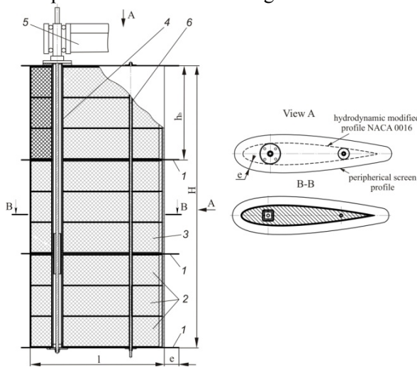
Figure 9. Blade construction.
